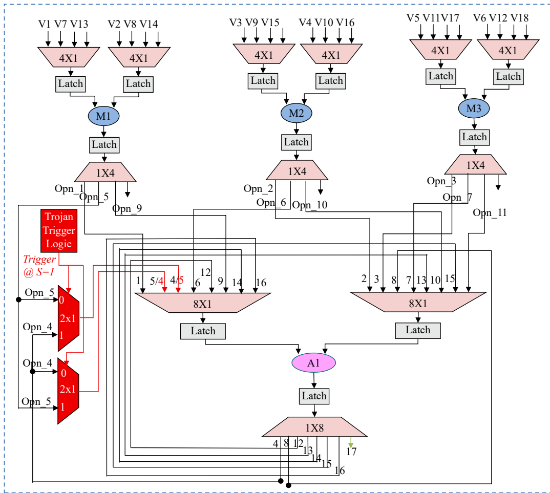
Fig. 4. SOT-HT induced CNN convolutional layer datapath
