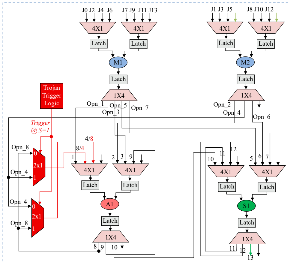
Fig. 5. SOT-HT induced IIR filter datapath
