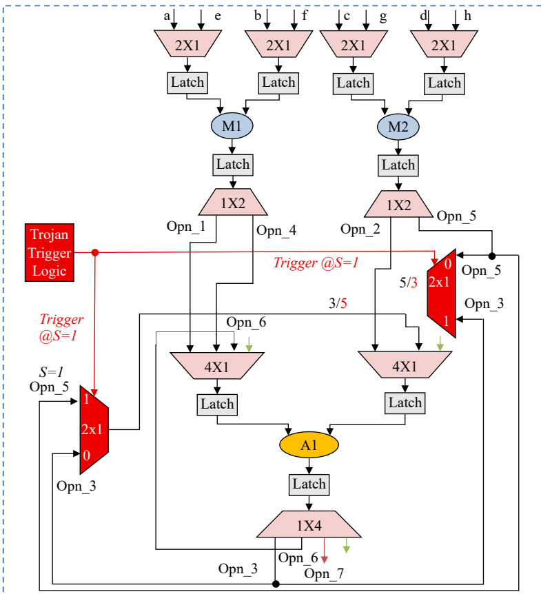
Fig. 1. SOT-HT induced 4-point DCT IP datapath
