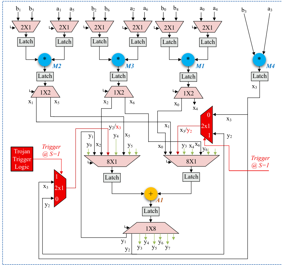
Fig. 3. SOT-HT induced FIR filter (UF=7) datapath
