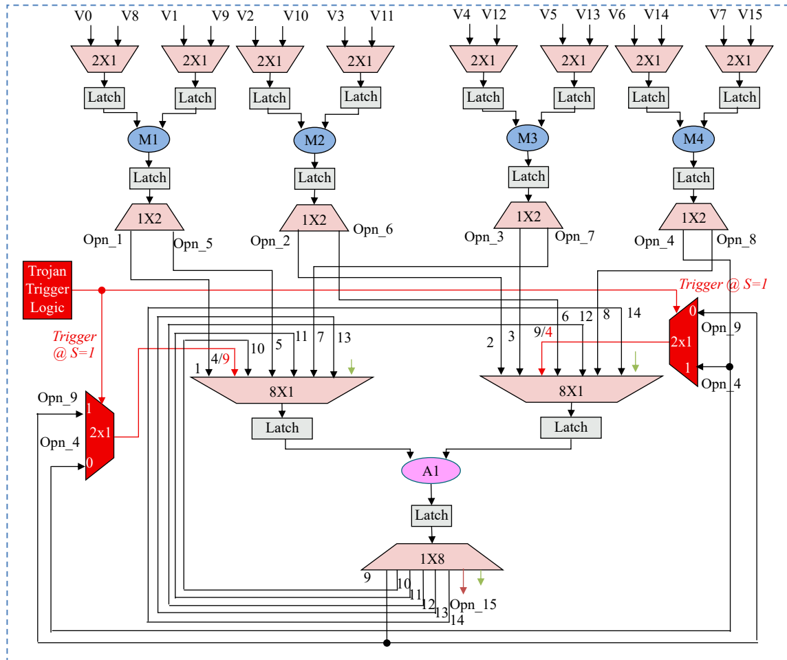
Fig. 2. SOT-HT induced 8-point DCT datapath
